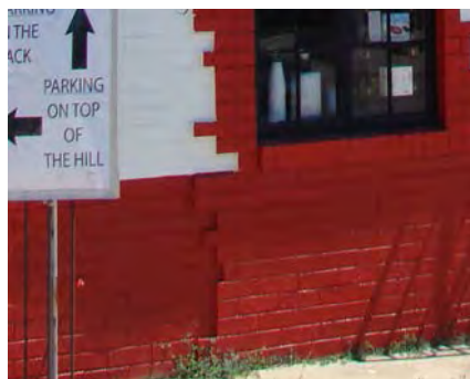
Above & Left: The exterior brick walls at 303 W. Main have severe step and sheer cracking.
