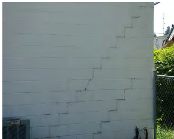
Right: Step cracking in the concrete block wall at 405 N. Broadway.
